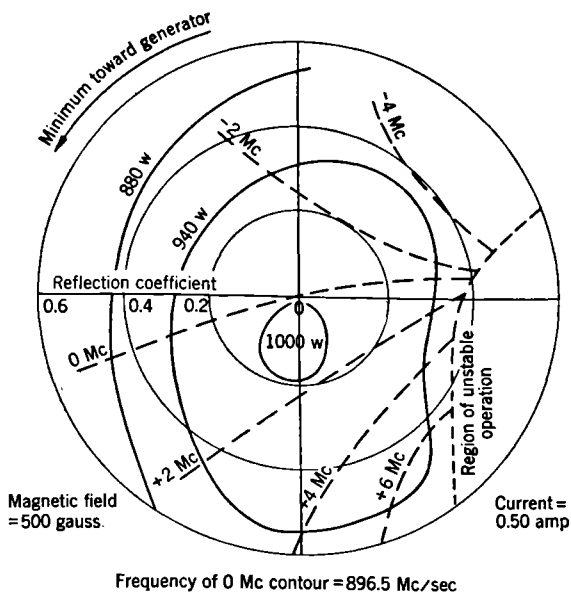
FIG. 19-4.—Rieke diagram for LCW magnetron.
